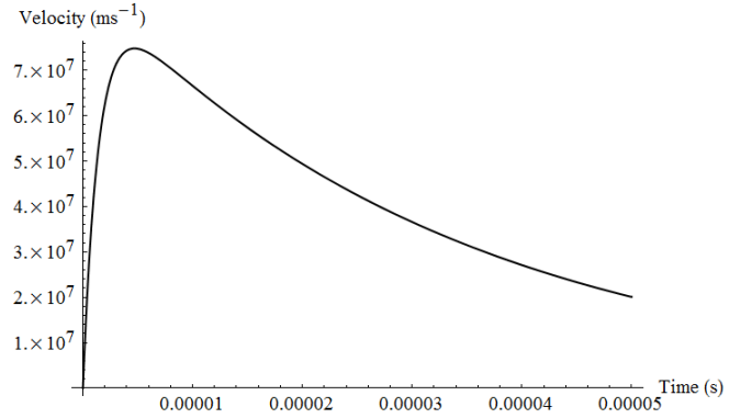
Figure 2: Velocity of RS-LC system with time.
