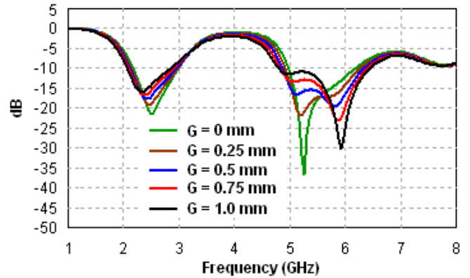
Figure 9: The S_{11} responses of the 3rd iteration Koch fractal monopole antenna of Figure 6(b) with G as the parameter
